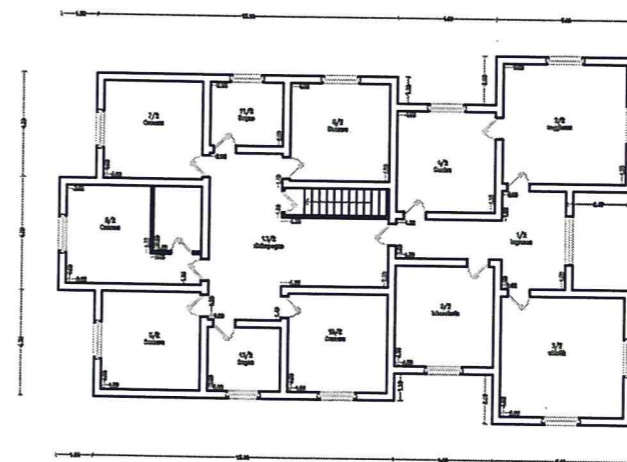
PIANO TERRA
